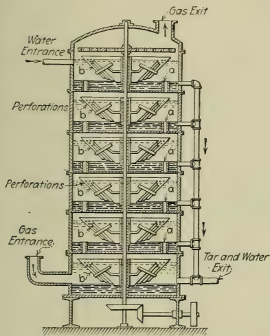
FIG. 65.—Feld Centrifugal Scrubber
